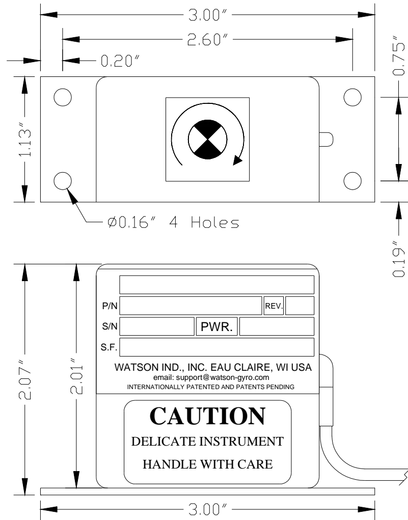
Figure 1: ARS-C122-1A Dimensions
