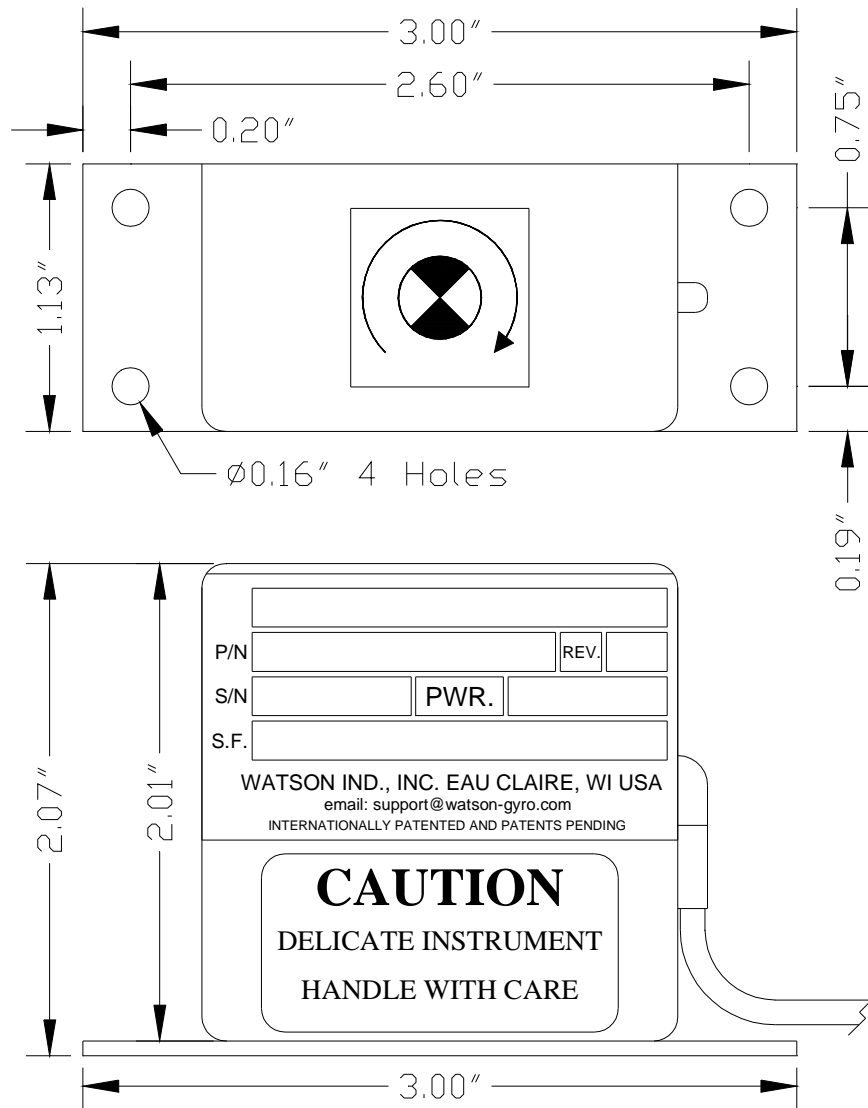
Figure 1: ARS-C132-1A Dimensions
