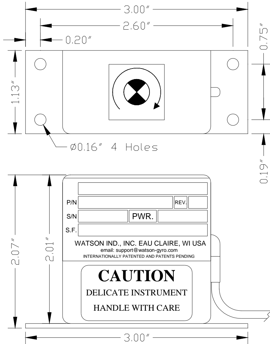
Figure 1: ARS-C142-1A Dimensions
