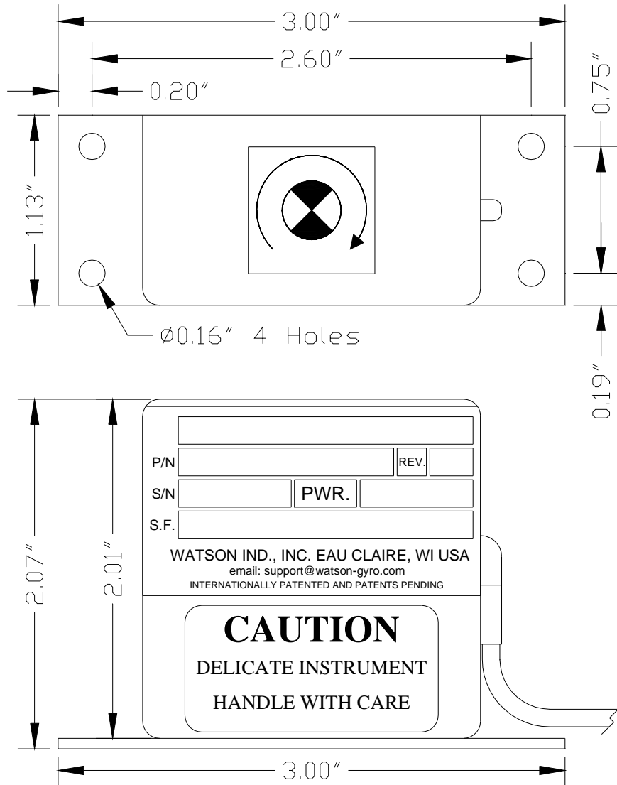
Figure 1: ARS-C152-1A Dimensions
