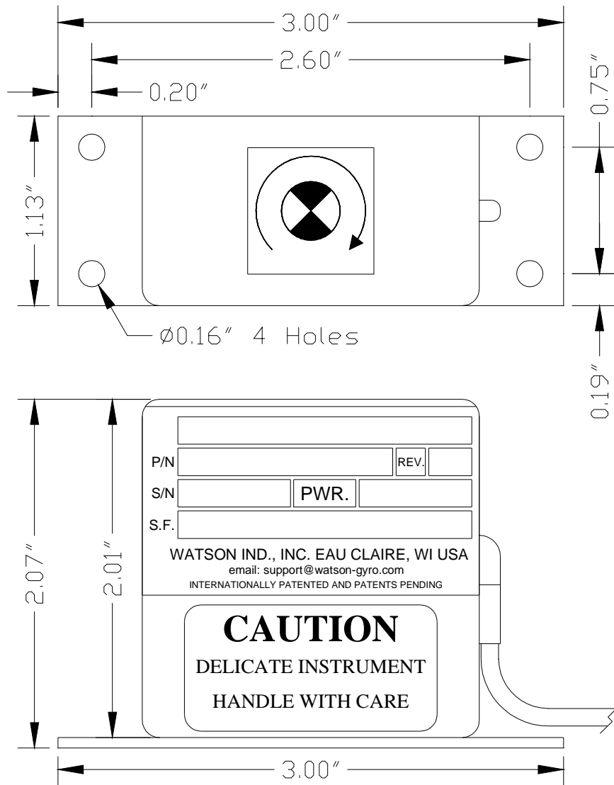
Figure 1: ARS-C122-1A Dimensions
